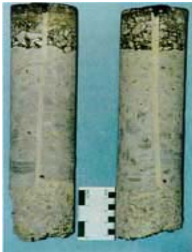
Figure 5. Pavement core reinstated in bus lane with Utilibond in 1995 still in perfect condition seven years later in 2002.
