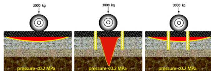
Uncut Road (Distributed Load) Conventional Pavement Cut (Concentrated Stress) Utilibond Reinstatement (Distributed Load)
